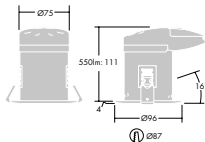
Fire rated adjustable
